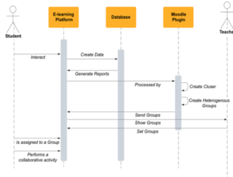
Gambar 4. Sequence Diagram [11]
