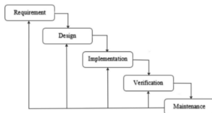
Gambar 1. Metode Waterfall [6]
